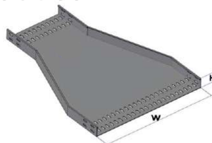
Cable Tray Straight Reducer 100 Height
