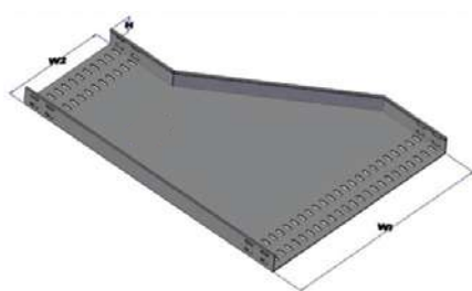
Cable Tray Left/Right Reducer 50 Height
