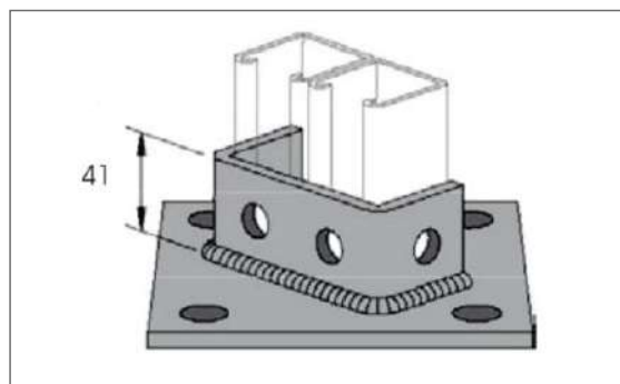
C-FHDCPBHDG/GU/SS-T Four Holes Double Channel Post Base
